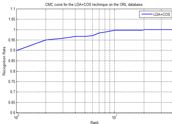
Fig.9 CMC curve for the LDA when no. of samples is 4.
