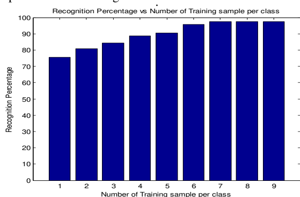
Fig.6 Recognition Percentage and Time for different no. of samples
