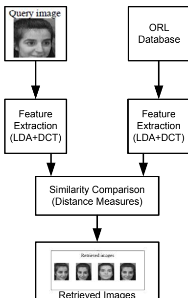
Fig.2 Block Diagram of LDA based Face Recognition
