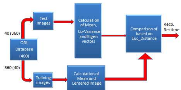
Fig.1 Block Diagram of PCA
