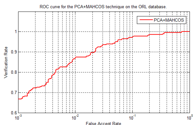
Fig.4 ROC curve for the PCA when no. of samples is 3.
