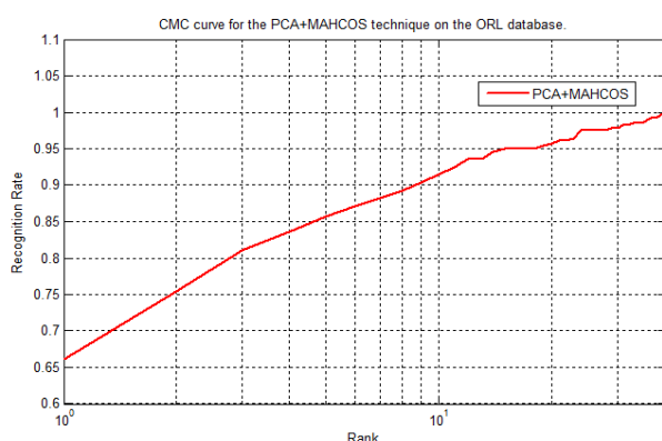
Fig.5 CMC curve for the PCA when no. of samples is 3.
