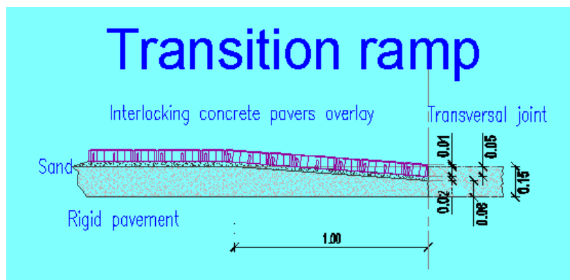
Figure 2. Rehabilitated pavement – existing pavement transition.
