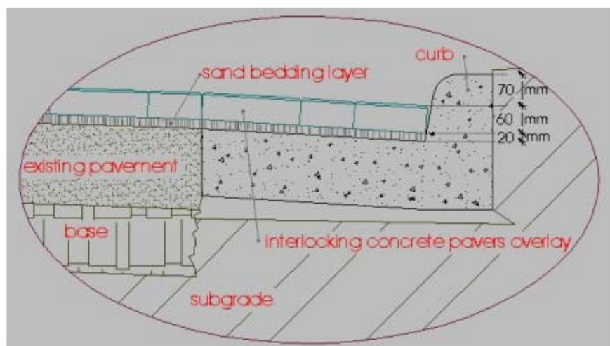
Figure 1. Cross sections. Overlay with concrete pavers.
