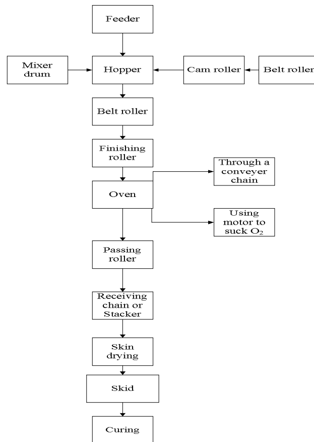
Figure 6.5: Sequence block diagram of pasting.
