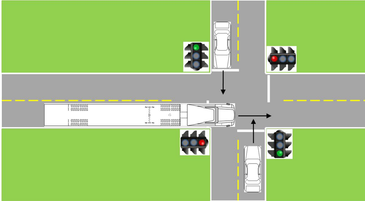
Figure 22. Running Red Light Crash Type
