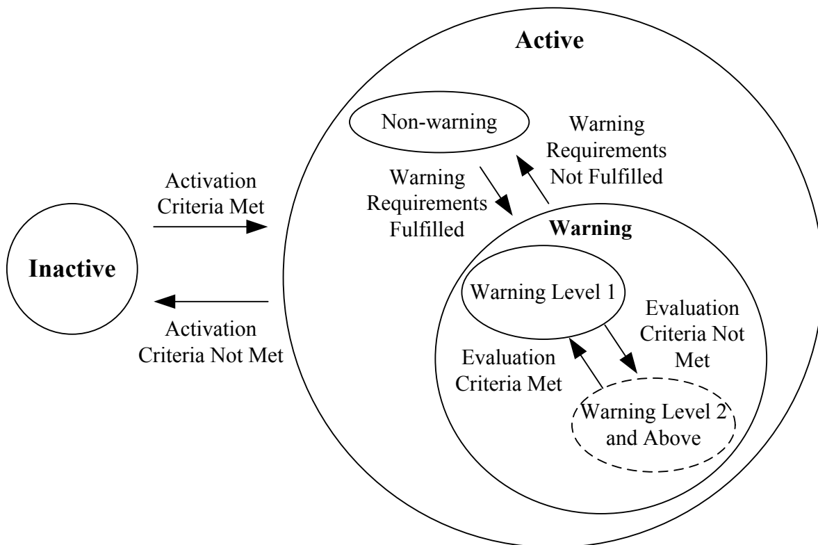
Figure 4. Side Collision Warning System Architecture (ISO 17387:2008)
