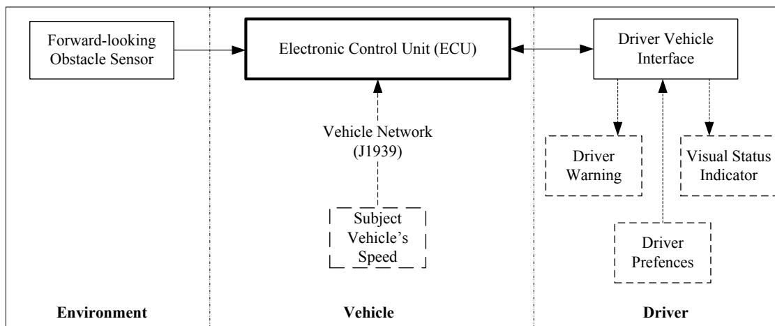
Figure 2. FCW System Architecture (Modified From ISO 15623: 2002)
