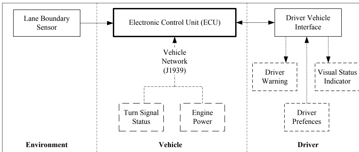
Figure 3. LDW System Architecture (Modified From Houser et al., 2005)
