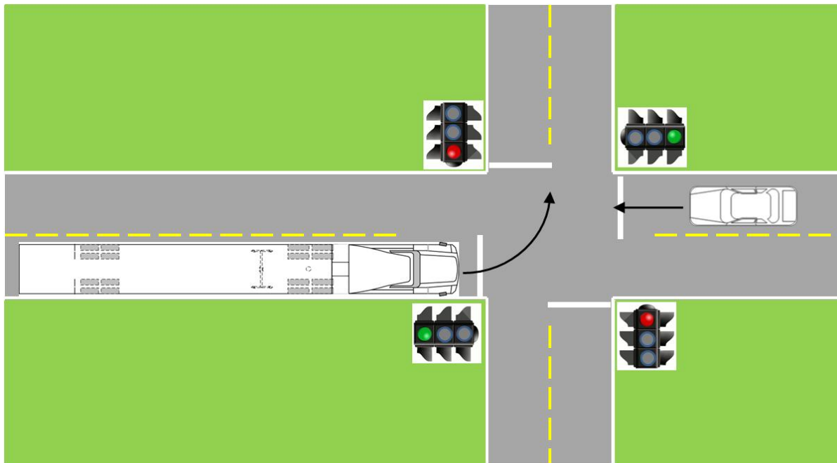
Figure 18. LTAP/OD at Signal Crash Type
