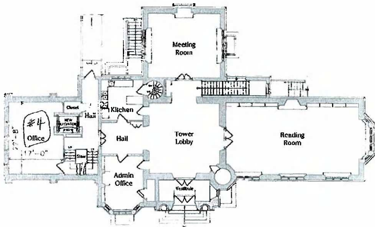
FIRST FLOORPLAN
