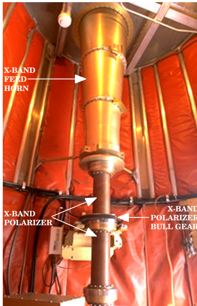
X-BAND FEED ASSEMBLY
