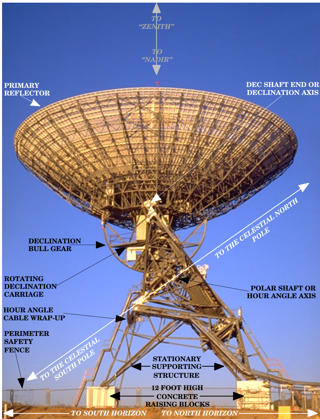
WEST-LOOKING VIEW OF THE GAVRT ANTENNA
