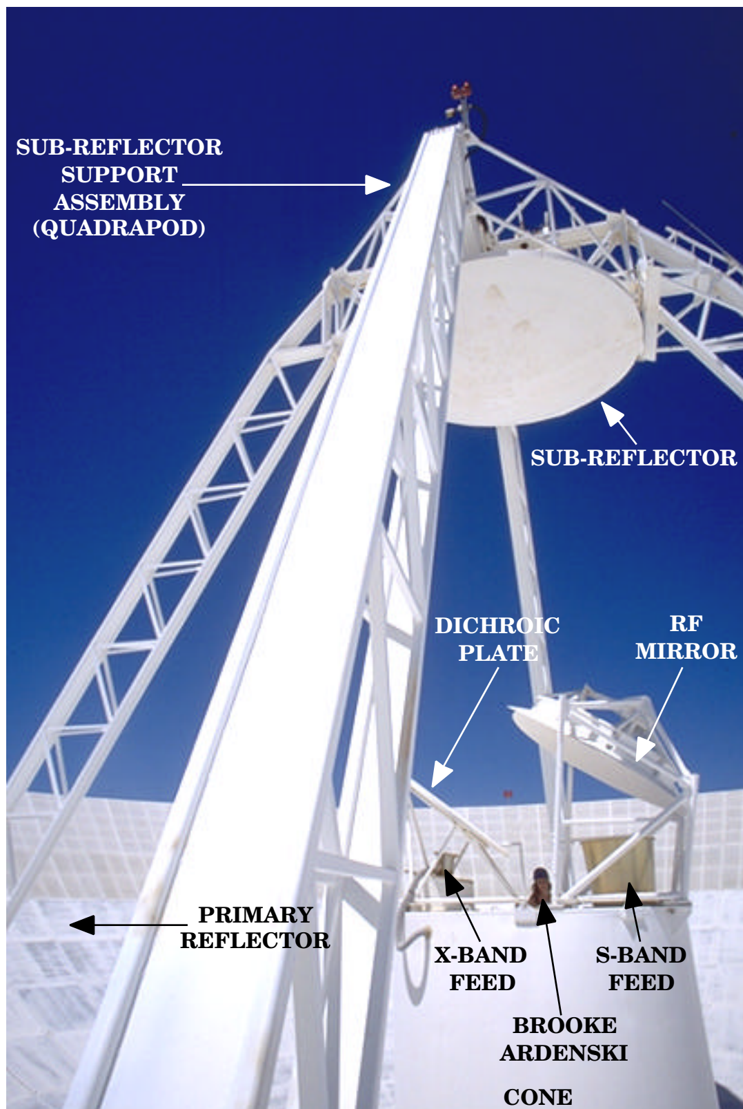
GAVRT ANTENNA SUB-REFLECTOR ASSEMBLY
