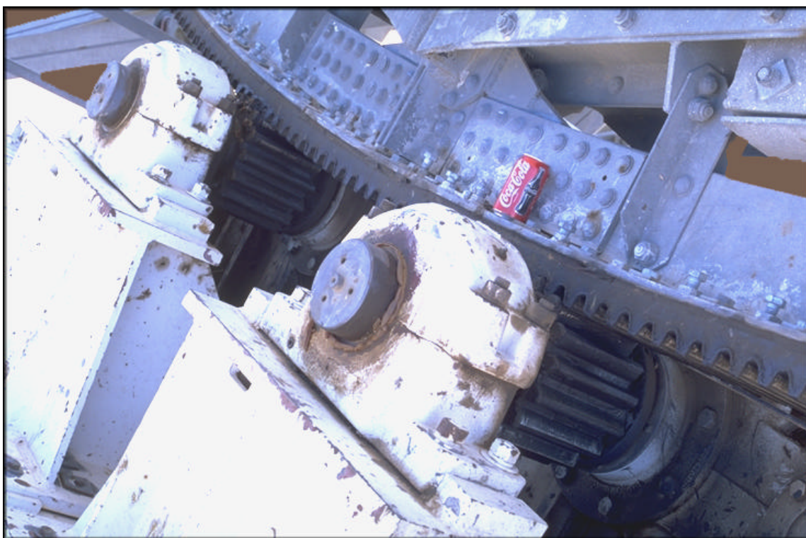
OUR ANGLE BULL GEAR AND PINION GEARS
