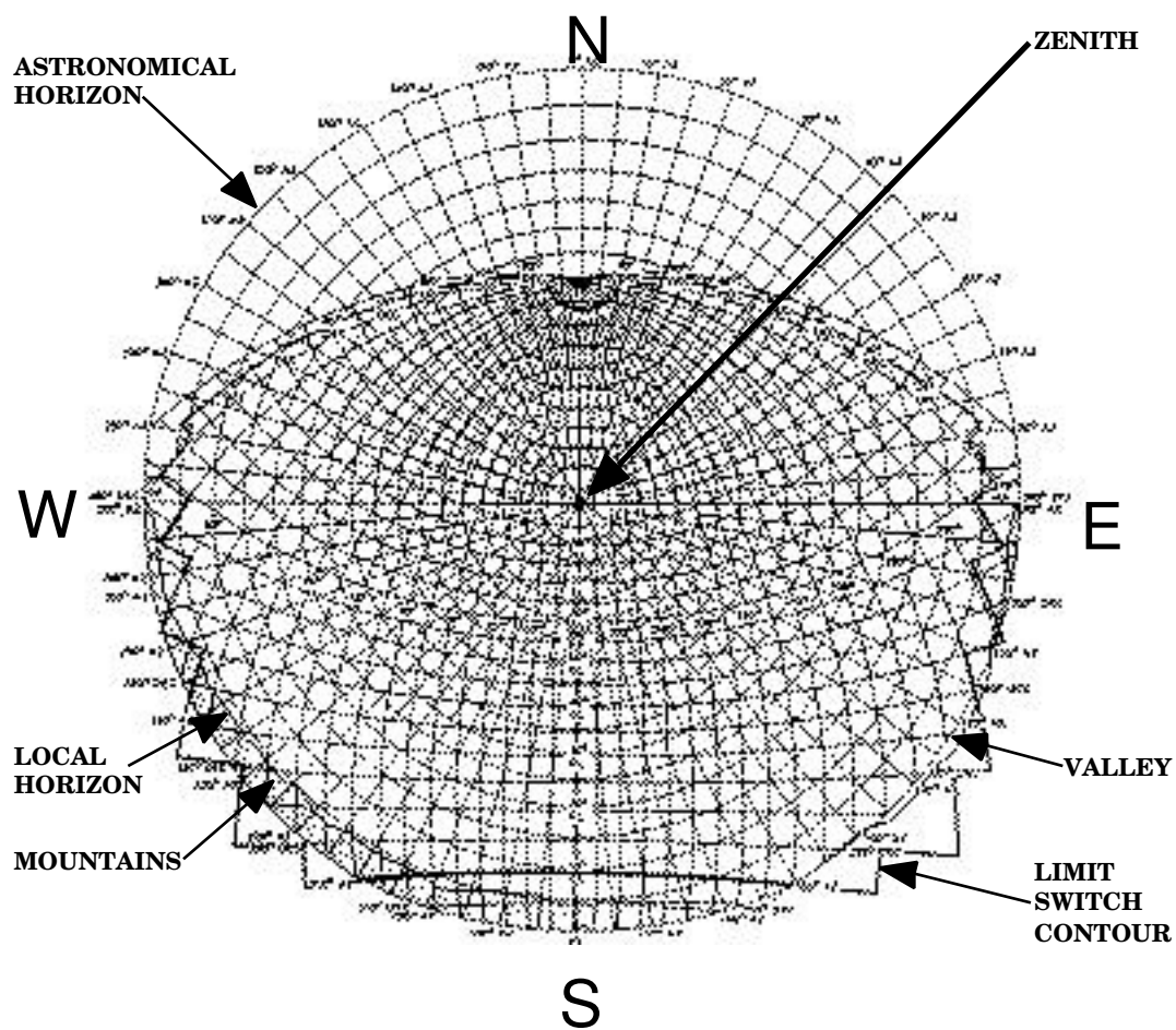
GAVRT ANTENNA HORIZON MASK
