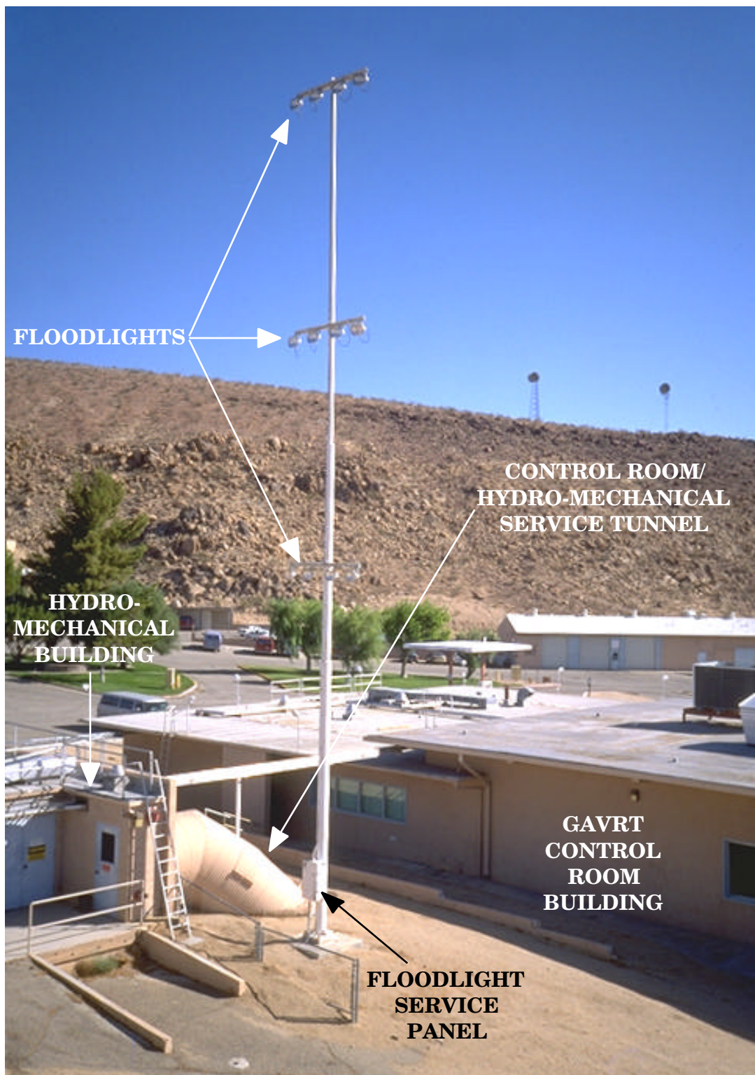
GAVRT ANTENNA FLOODLIGHTS & CONTROL ROOM BUILDING
