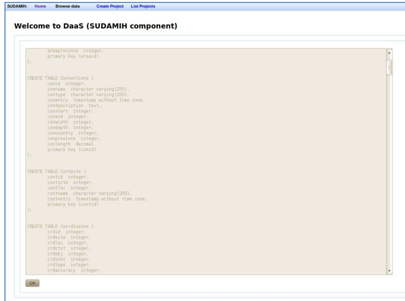
Component 2 – Access Database converter (test screenshot – user does not see code generated)
