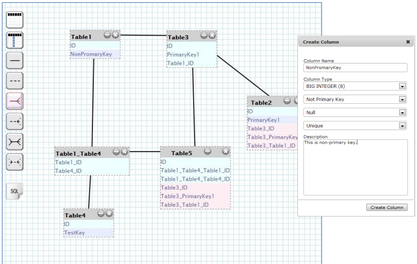
Component 3 - Graphical SQL-designer for structuring relational databases
