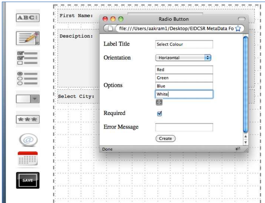
Component 4 – Form-builder utility
