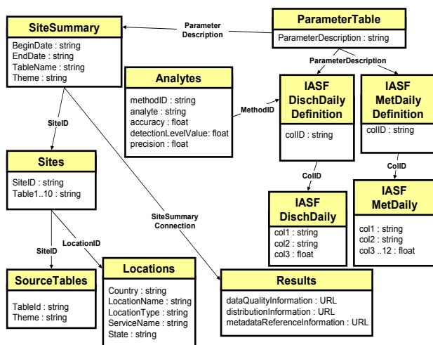
Figure 4 – Ontology for STEWARDS Data Archive
