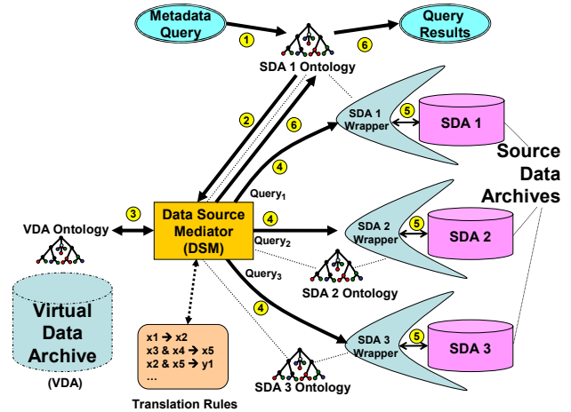
Figure 1 – Metadata Integration Framework: (1) Metadata query is issued using terms from SDA#1 ontology. (2) Query is transmitted to DSM, which uses translation rules to reformat query in terms of the VDA ontology (3). DSM translation rules next rewrite VDA query in terms of SDA#2 and SDA#3 ontologies, and queries for all three SDAs are sent to their respective wrappers (4). Finally wrappers query the SDAs archives to retrieve metadata (5) and transmit results back through DSM (6), which translates results back into the SDA#1 ontology language.
