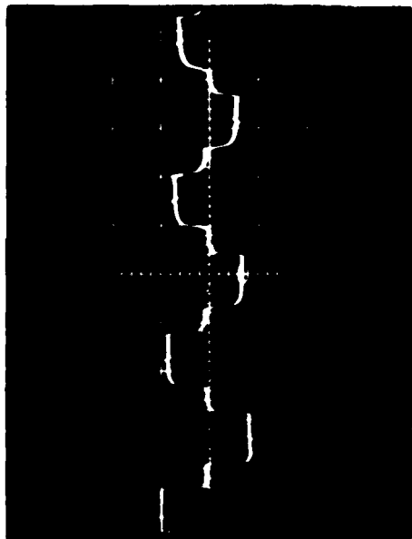
Figure 4. Open-Circuit Waveforms From Coaxial-Cable Arrays. Time scale is uncalibrated. (a) Z_2 = Z_1 . (b) Z_2 = 3Z_1 . (c) Z_2 = Z_1/3 .
