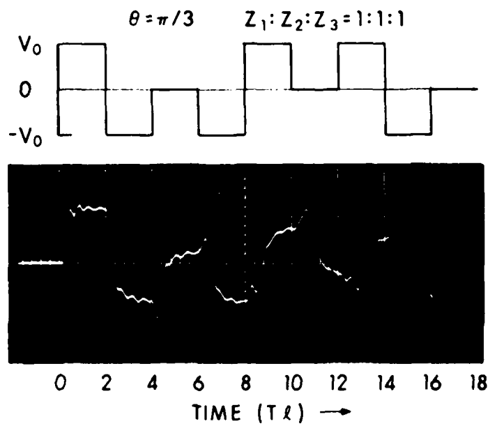
Figure 18. Predicted and Observed Waveforms for Z_1:Z_2:Z_3 = 1:1:1 .
