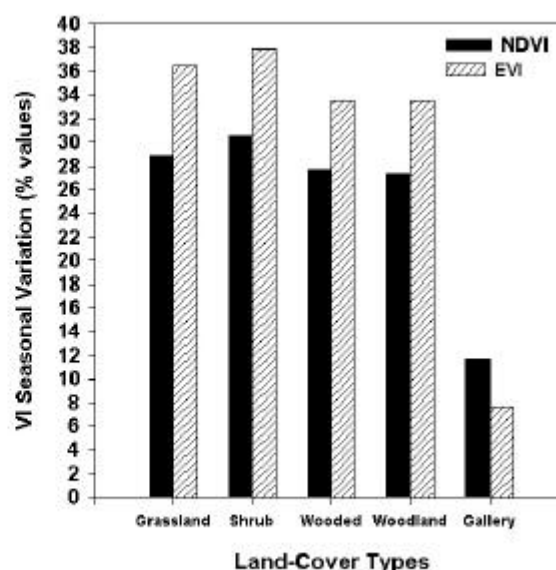
Figure 4 - NDVI & EVI Seasonal Variation
