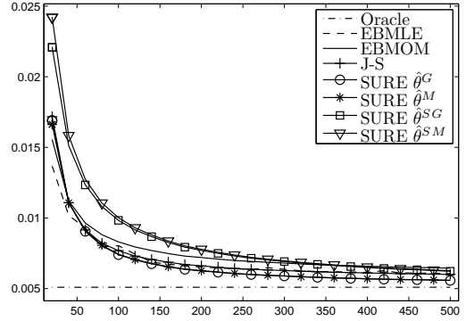
(4) A \sim \text{Inv-}\chi^2_{10} , \theta = A ; X \sim N(\theta, A) .
