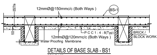
DETAILS OF BASE SLAB - BS1 SCALE 1:30
