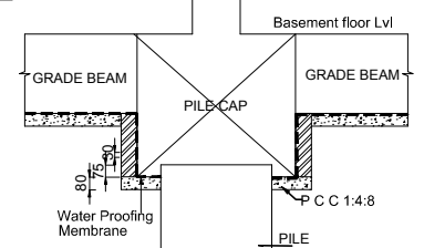
TYPICAL SECTION OF SINGLE PILECAP SCALE 1:25
