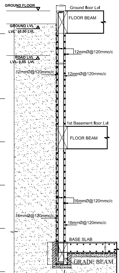
RETAINING WALL SECTION A-A
