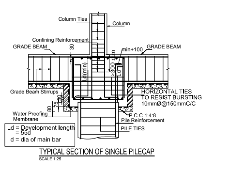
TYPICAL SECTION OF SINGLE PILECAP SCALE 1:25
