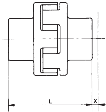
Axial misalignment
