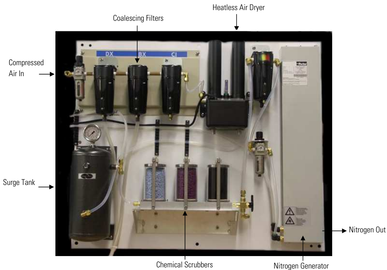
Figure 1–10. Zero Air Panel System with Nitrogen
