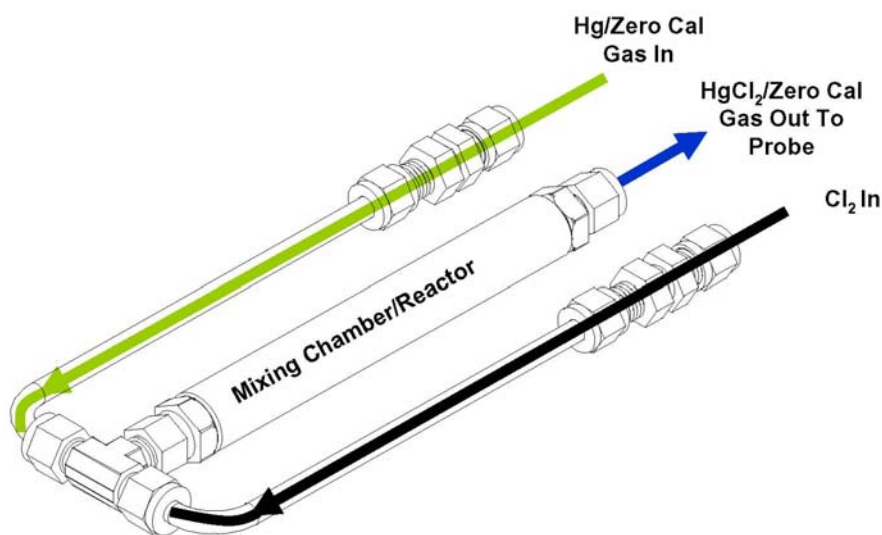
Figure 1–6. Oxidizer Flow Diagram
