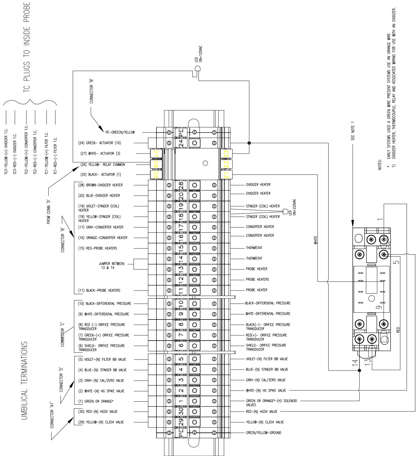
Figure B-13. Model 83i with Oxidizer Terminal Block Wiring Diagram 105507-00
