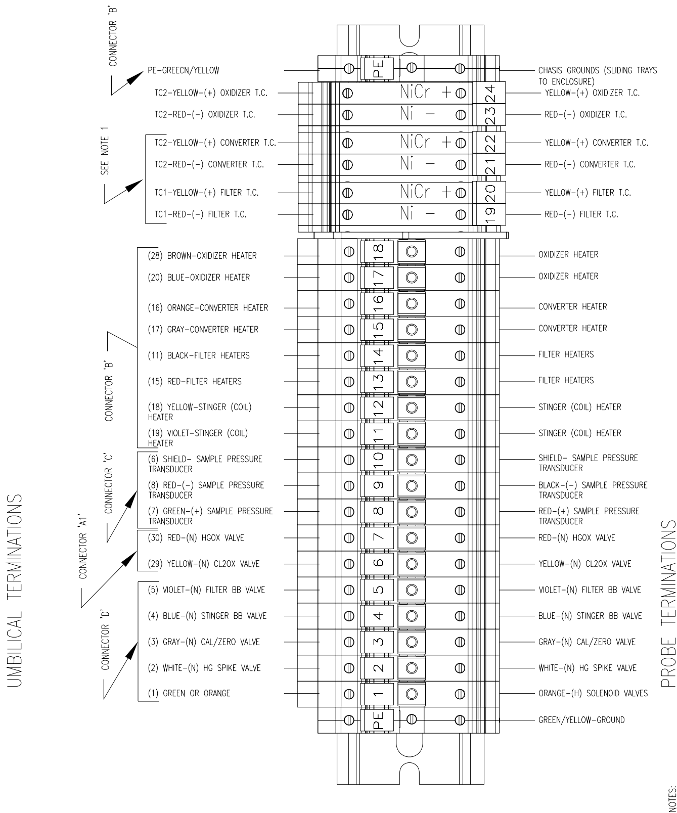
Figure B-11. 83i GC with Oxidizer Terminal Block Wiring Diagram 104734-00
