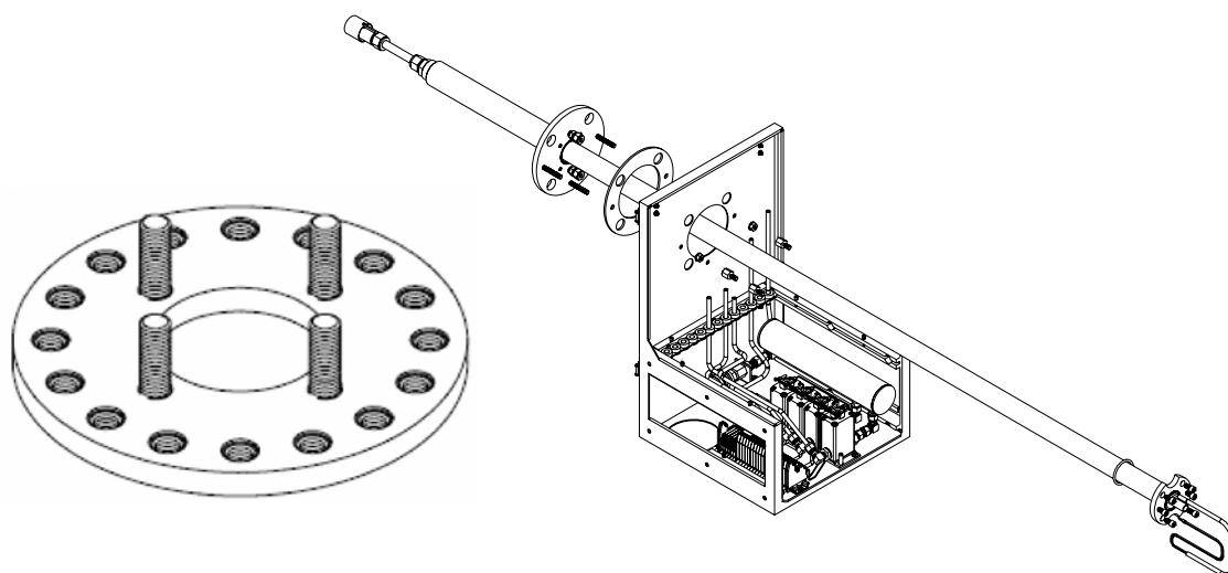
Figure 1-12. Stack Mounting Flange
