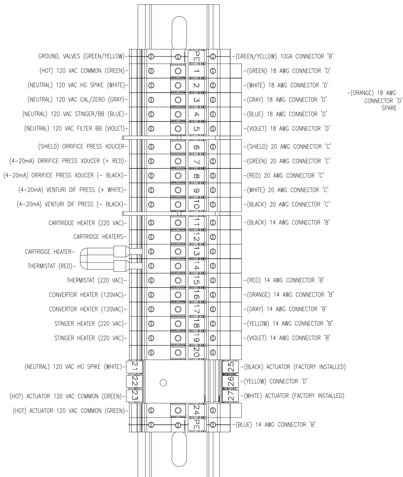
Figure B-10. 83/Terminal Block Wiring Diagram 104588-00
