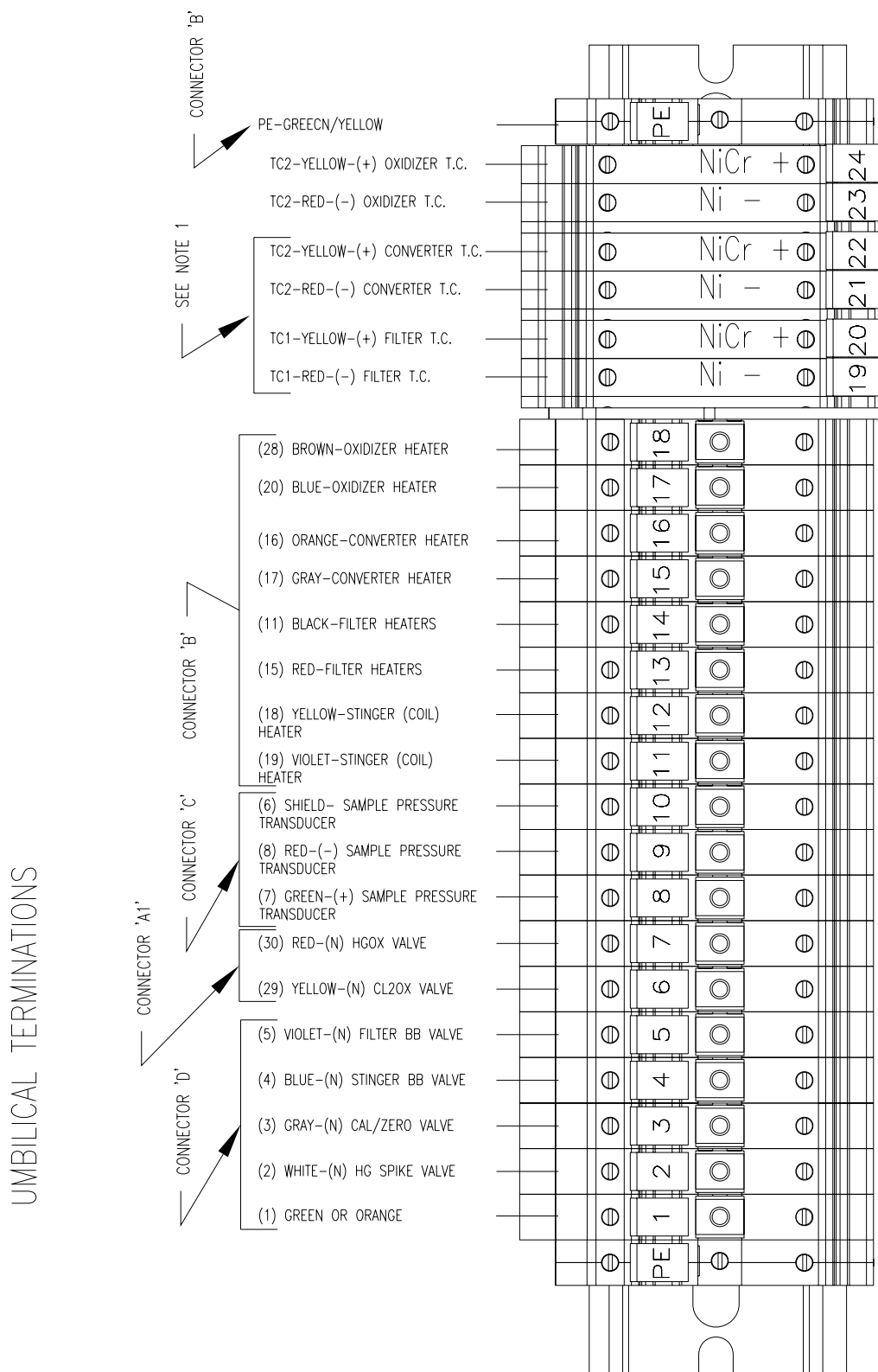
Figure B-12. Umbilical Wiring Detail
