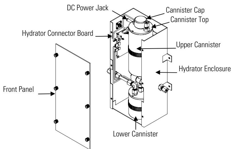
Figure 1–9. Hydrator Components
