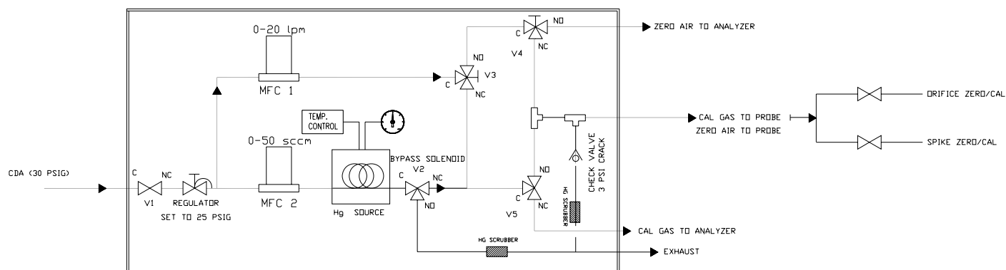
Figure 1-2. Model 81i Flow Diagram
