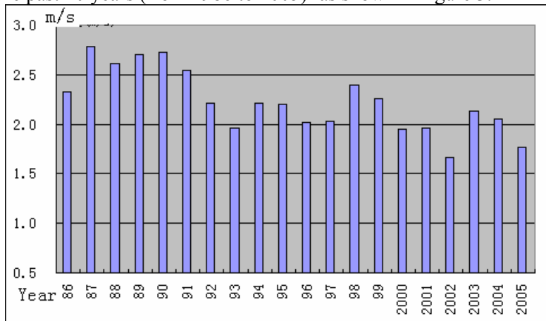
Figure 3 The annual average wind speed in the local meteorological station Therefore the probability that PLF is 6.8% higher than the estimated value throughout the whole project operation period is unreasonable. The proposed project is always lack of financial attractiveness.
