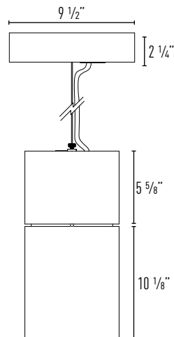
Aircraft Cable with DMX Dimming
