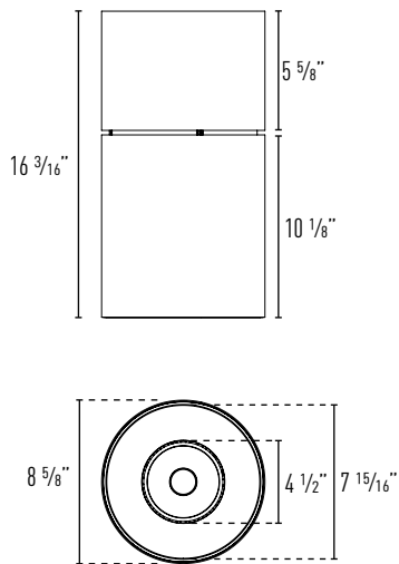
Surface Mount
