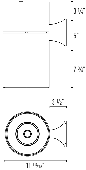
Wall Mount
