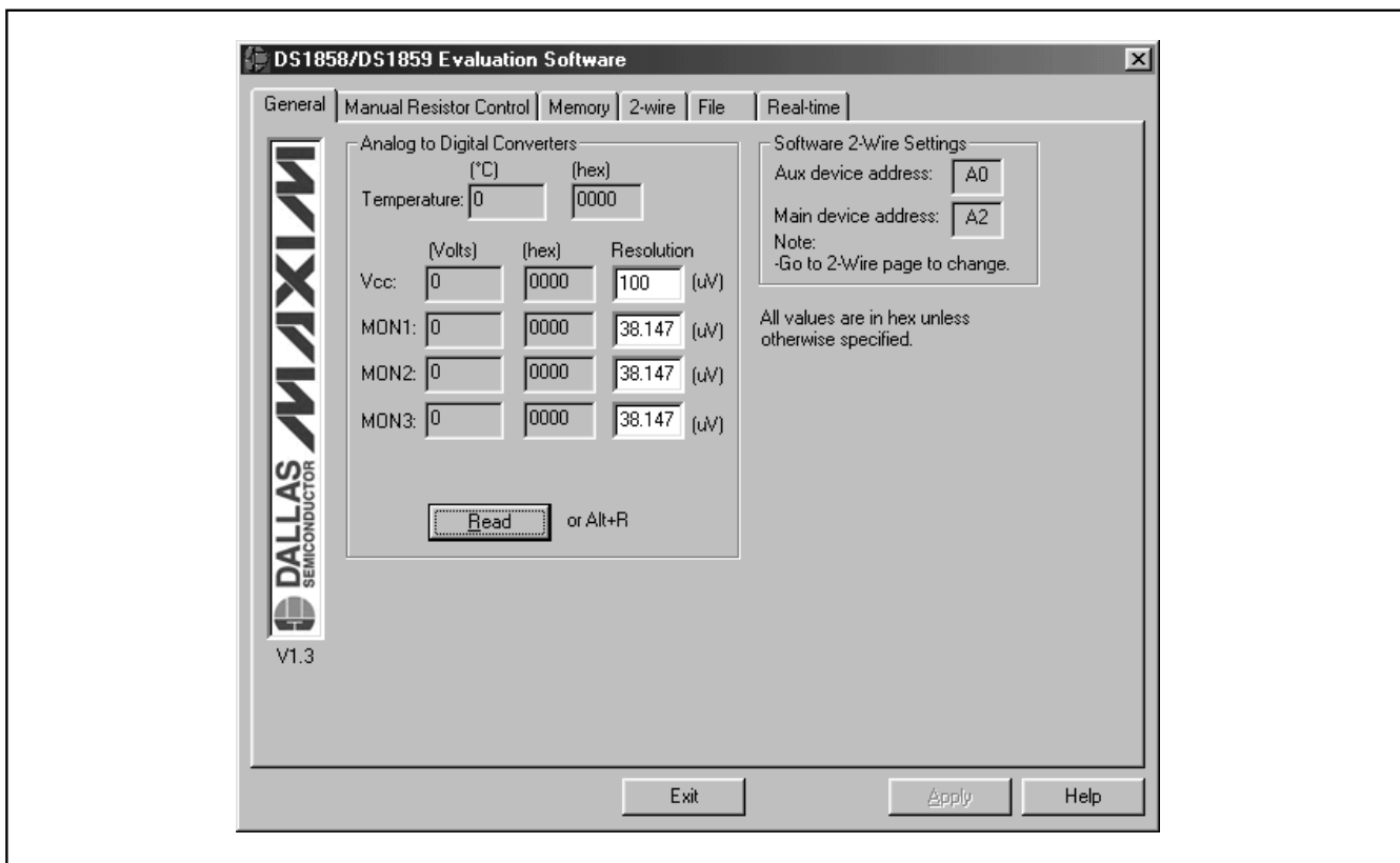
Figure 6. General Page
