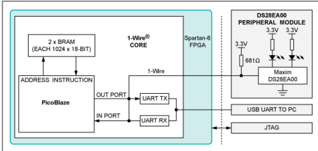
Figure 1. System design block diagram.
