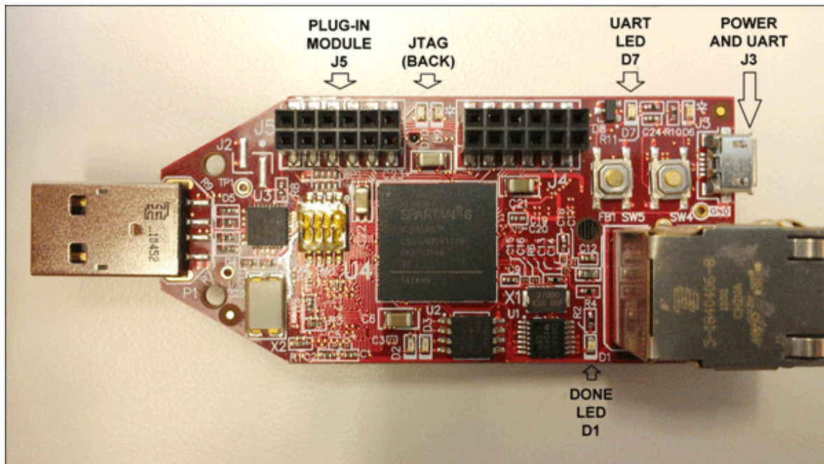
Figure 2. The S6LX9 MicroBoard.
