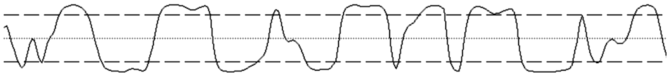
JMA double stochastic
