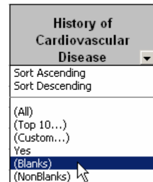
Figure 8. Excel AutoFilter
