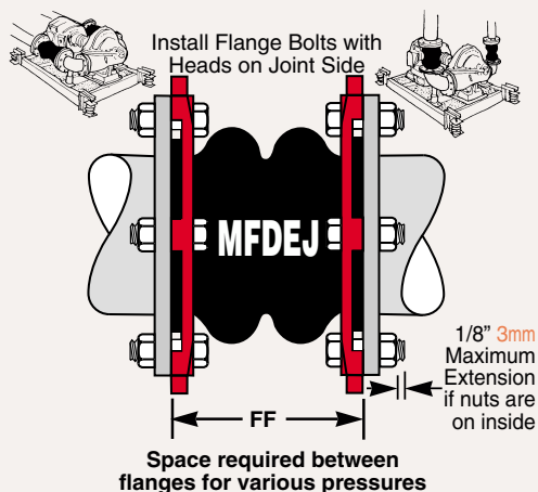
MASONFLEX MFDEJ Pressure Extension Table
