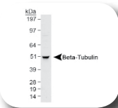
Detection of Beta-Tubulin in HeLa whole cell lysate using NB600-936.
