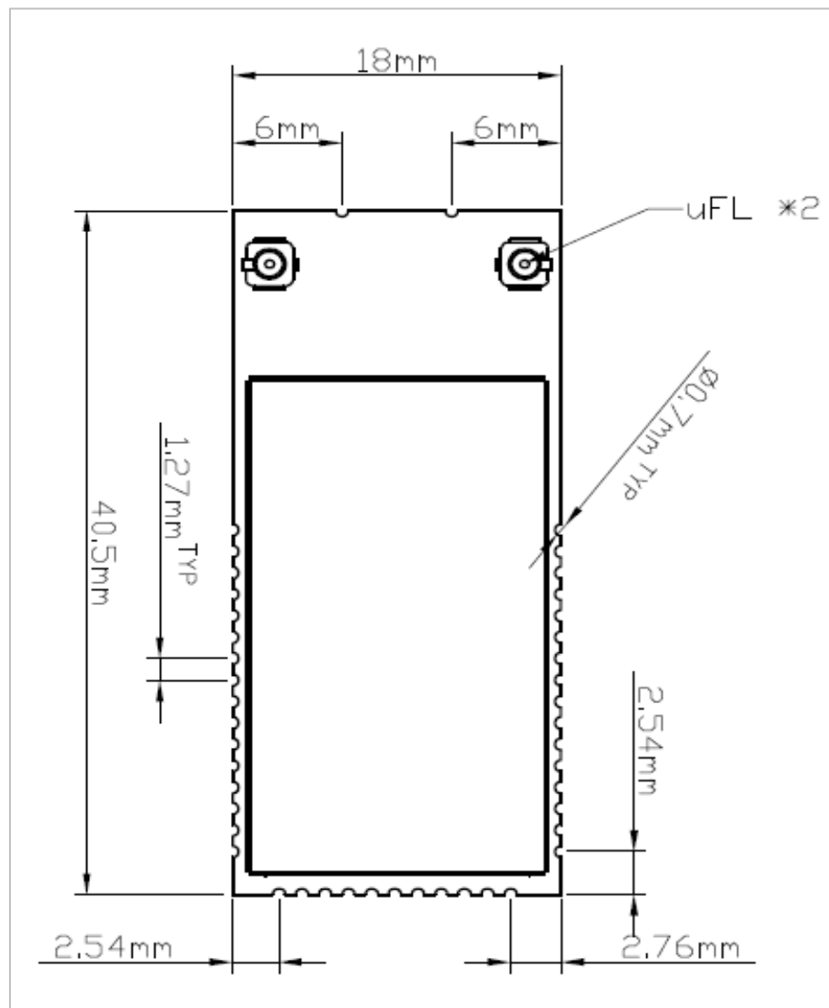
Figure : MD-223FA Outline Drawing
