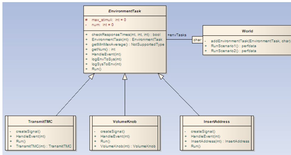
Figure A.2: Overview of the World and Environment Classes
