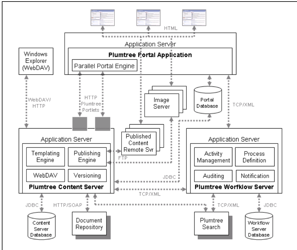
Figure 2-1: Publisher Architecture
