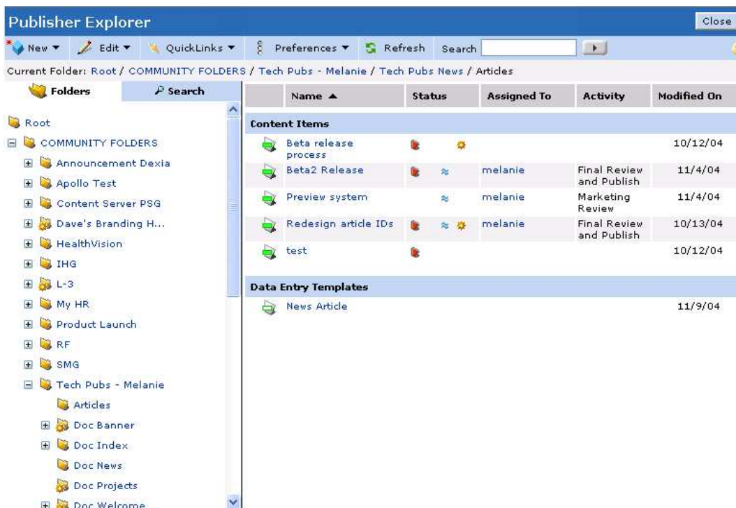
Figure 3-1: Publisher Explorer
