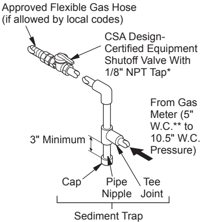
Figure 4 - Gas Connection
