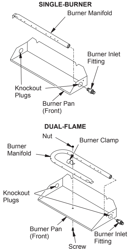
Figure 6 - Installing Burner
