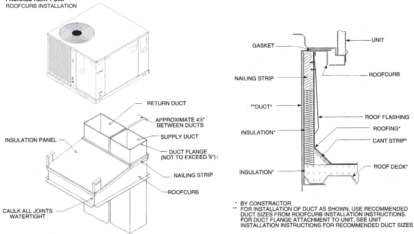
FIGURE 5 PACKAGE HEAT PUMP ROOFCURB INSTALLATION
