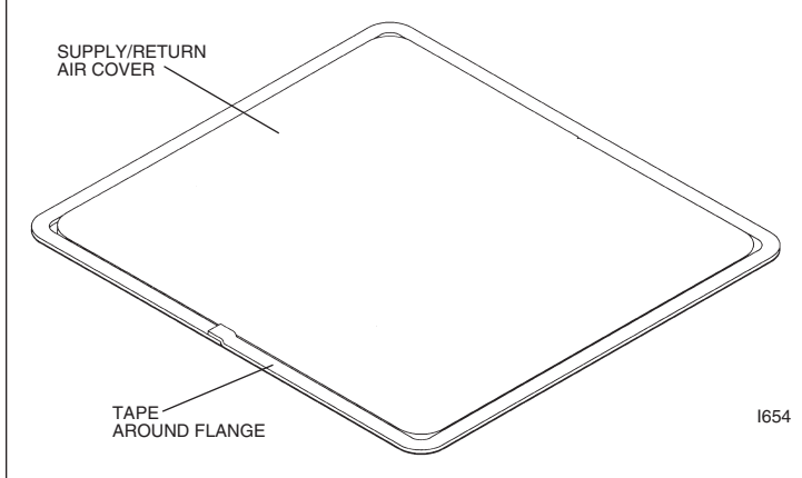
FIGURE 8 COVER GASKET DETAIL FOR UNITS SHIPPED FOR SIDE DISCHARGE APPLICATION BEING CONVERTED TO DOWNFLOW
