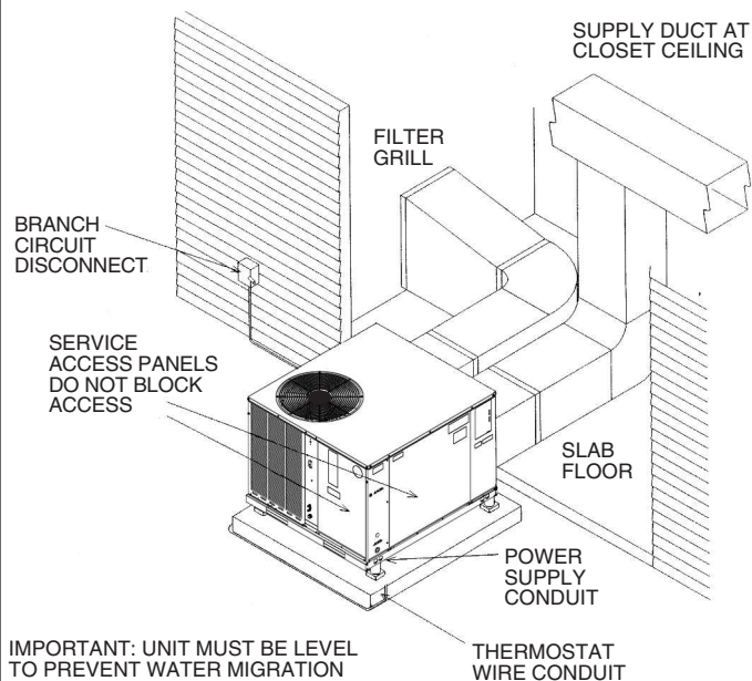
FIGURE 3 PACKAGE HEAT PUMP OUTSIDE SLAB INSTALLATION, CLOSET DISTRIBUTION SYSTEM. SLAB FLOOR CONSTRUCTION
