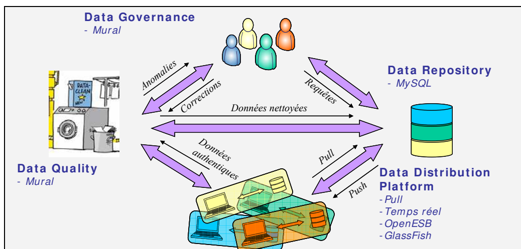
Figure 15 : SumEHR: Infrastructure Open Source
