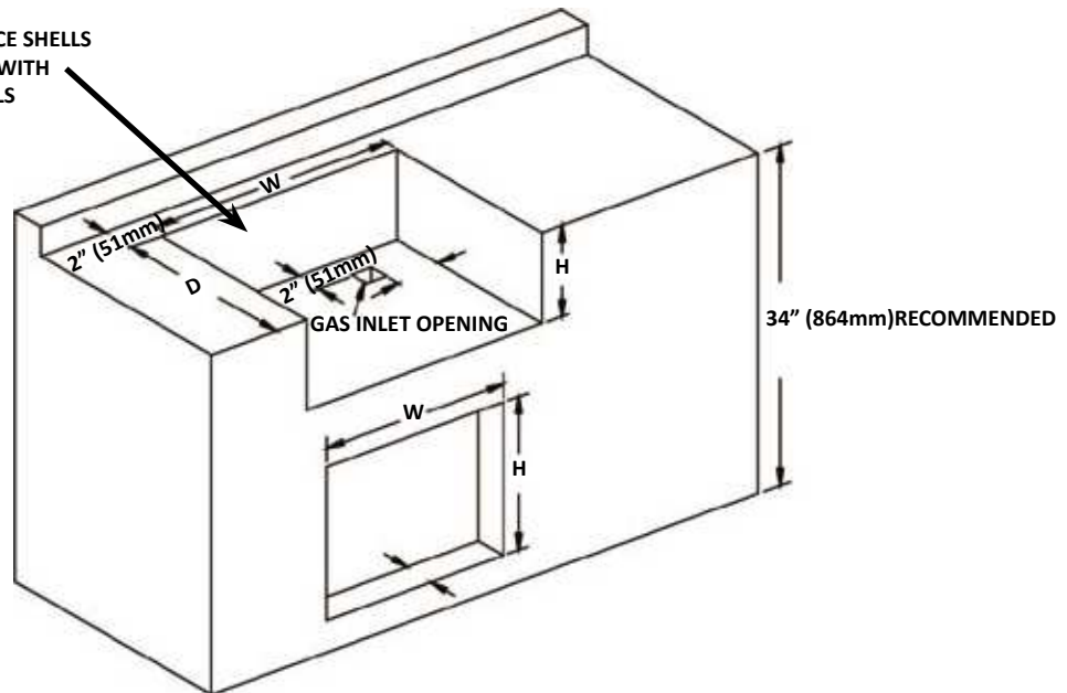
OPENING DIMENSIONS
