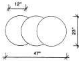
Three Cabinet Crescent Set: Round 23" diameter with two crescents
