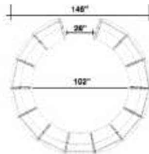
Curving Kiosk 146" diameter, 13 sections 22" x 146" with risers, 13 sections--open back
