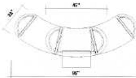
Oval Curving Multi-Level Computer Cabinet 22" x 96" with one brace panel, 3 sections--open back
