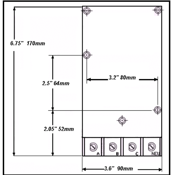
Figure 4.3 Power Module Dimensions
