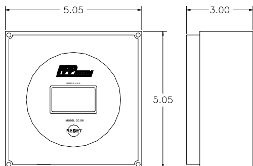
NEMA 4X Enclosure
