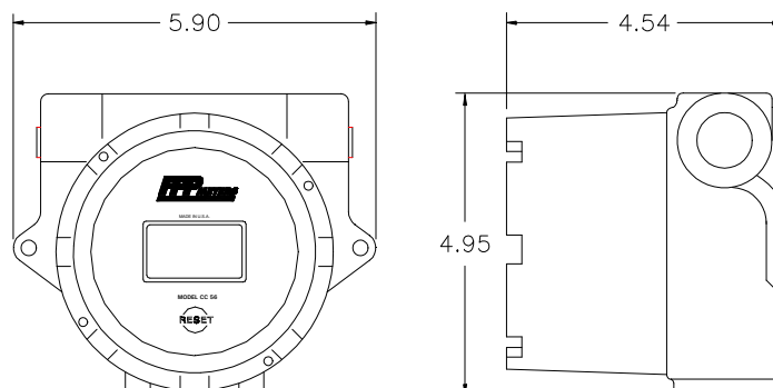
NEMA 7/4 Enclosure
