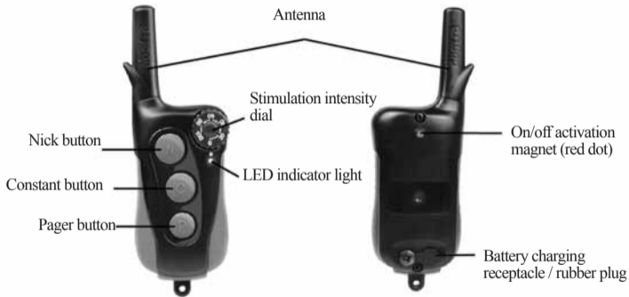
Transmitter
