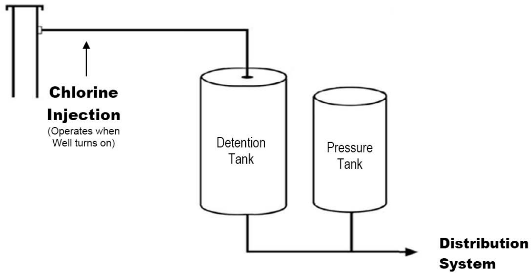
FIGURE 4.1 - DISINFECTION
