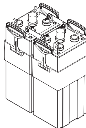
SINGLE CELL (1RE) CONNECTIONS
