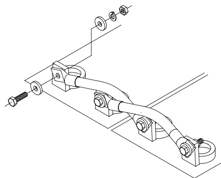
6 – CELL (6RE) Figure 1.2
