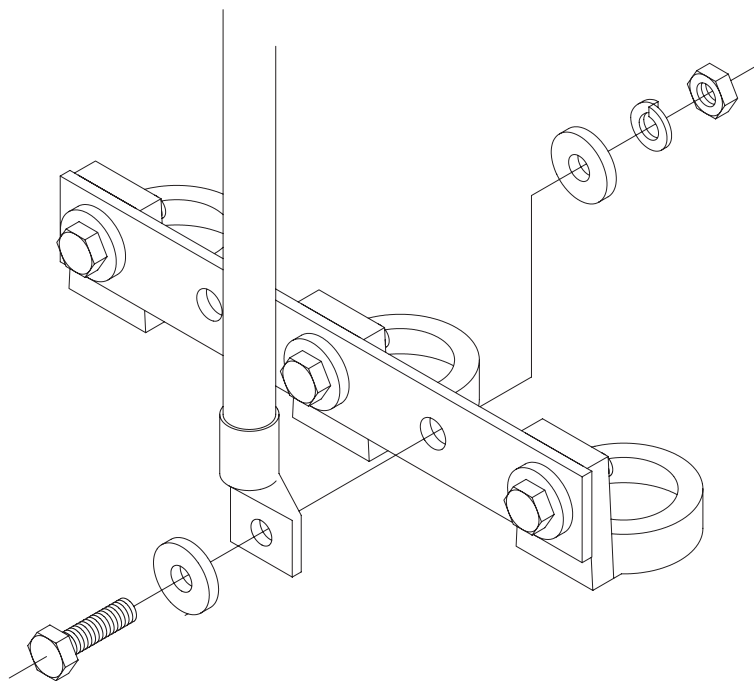
TERMINAL PLATE INSTALLATION
