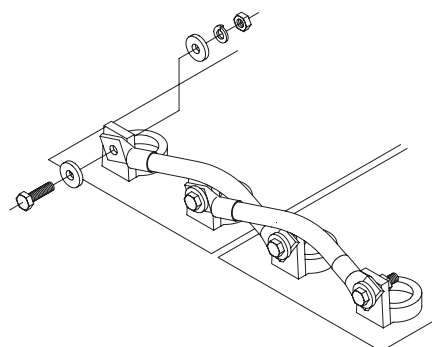
MULTI CELL UNITS (6RE) CONNECTIONS
