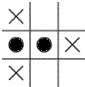
Figure 6.1, Tic-Tac-Toe Board
