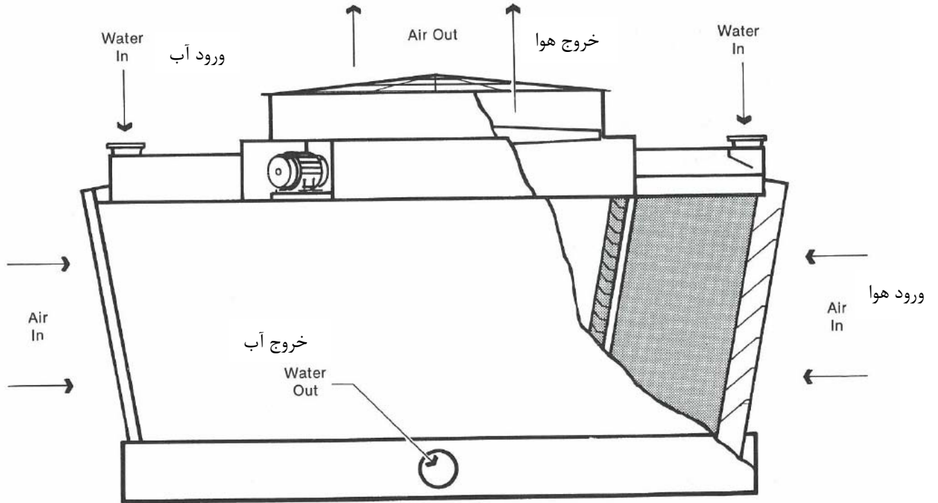
Fig. 4- INDUCED CROSSFLOW TYPE COOLING TOWER
