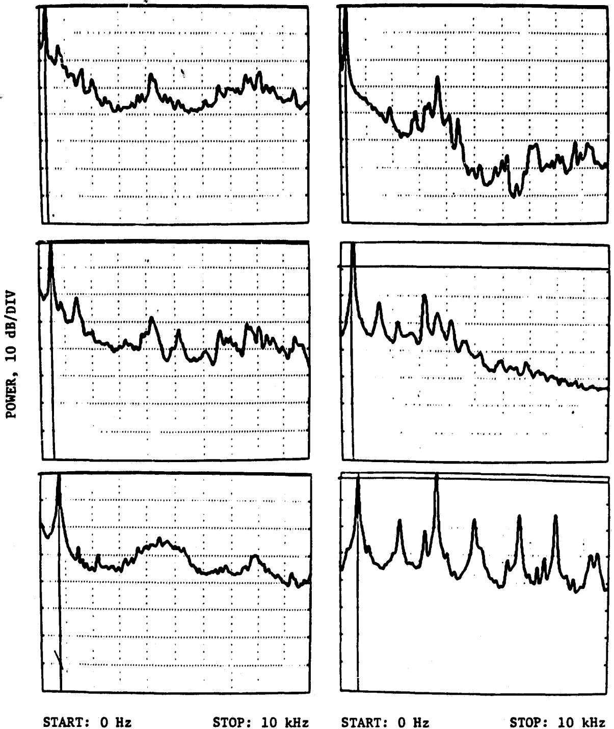
Figure 28. The three spectra on the left side are from vane 39 at average flow velocities of 12.1, 23.5 and 36.2 m/s from top to bottom. The three spectra on the right are for vane 42 at average flow velocities of 11.1, 24.0 and 32.5 m/s, top to bottom.
