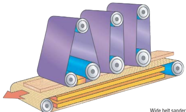
Wide belt sander
