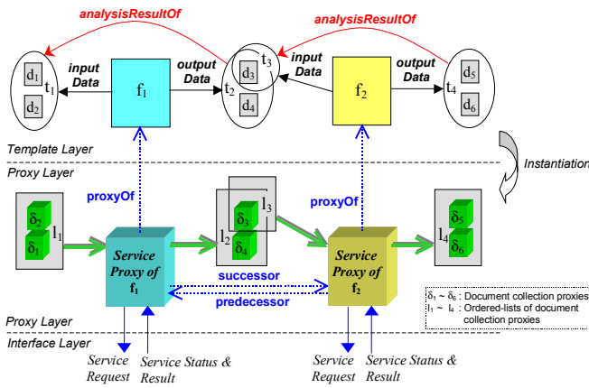
Fig. 4. Instantiation of a template by creating proxies
