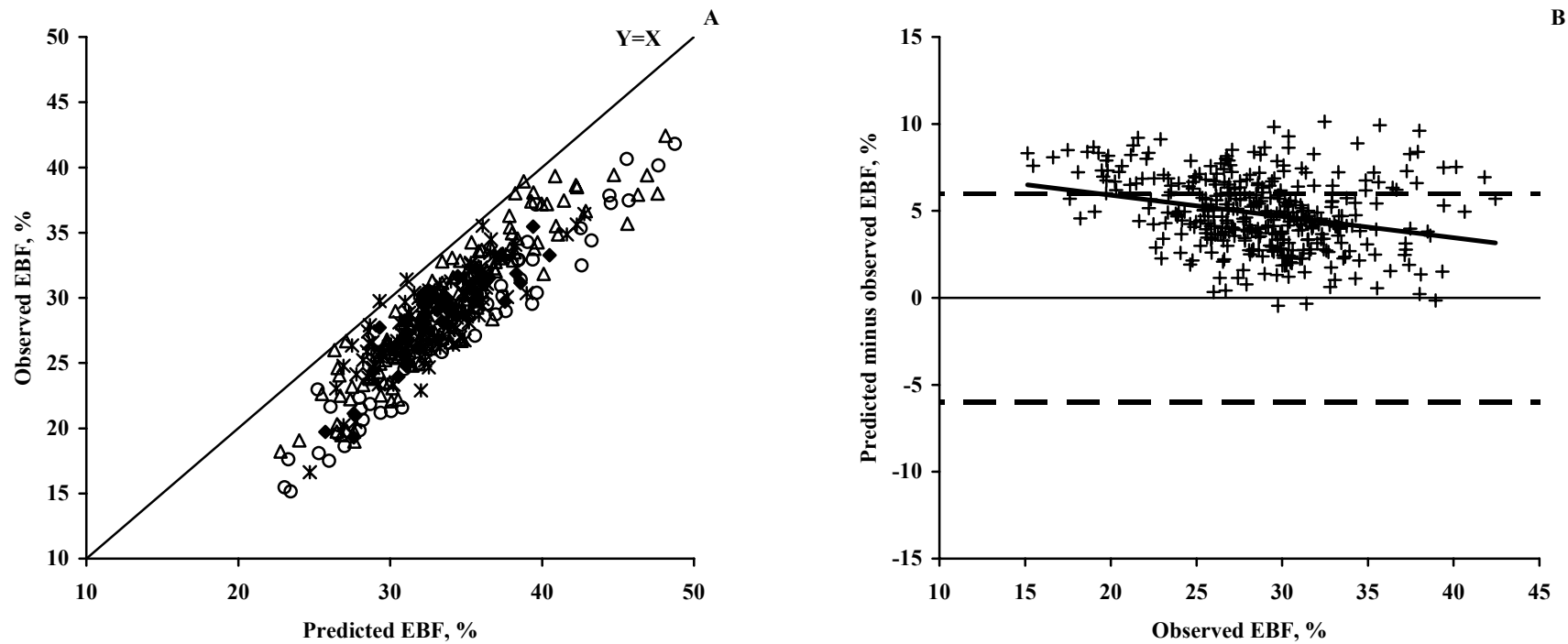
Figure 5. Prediction of empty body fat (EBF, % of empty body weight) at the end of the feeding period using the day-step model simulation. (A) Relationship between observed and predicted EBF. The data points are from Nour and Thonney (1987), \Delta ; Perry and Fox (1997), o; Perry et al. (1991), *; and Guiroy (2001), \blacklozenge . The regression is Y = -2.38 + 0.93 \times X with N = 358 animals, r^2 = 0.81 , and bias = -14.4% ( P < 0.05 ). Intercept and slope are different from zero and unity, respectively ( P < 0.05 ). (B) Deviation (predicted minus observed) vs observed FSBW indicated that 71% of the points lie within \pm 6\% (dotted lines). The solid line shows a systematic bias.
