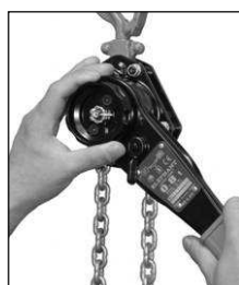
5) Hold down the feed handle softly and manipulate the operation handle to pull the bottom hook.
