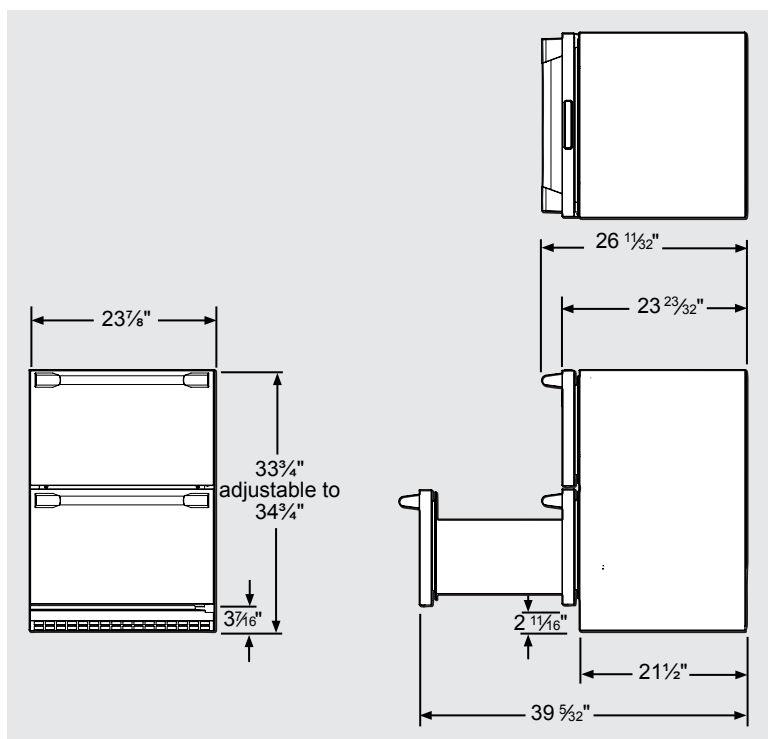
Product Dimensions
