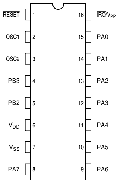
Figure 1. Pin Assignments
