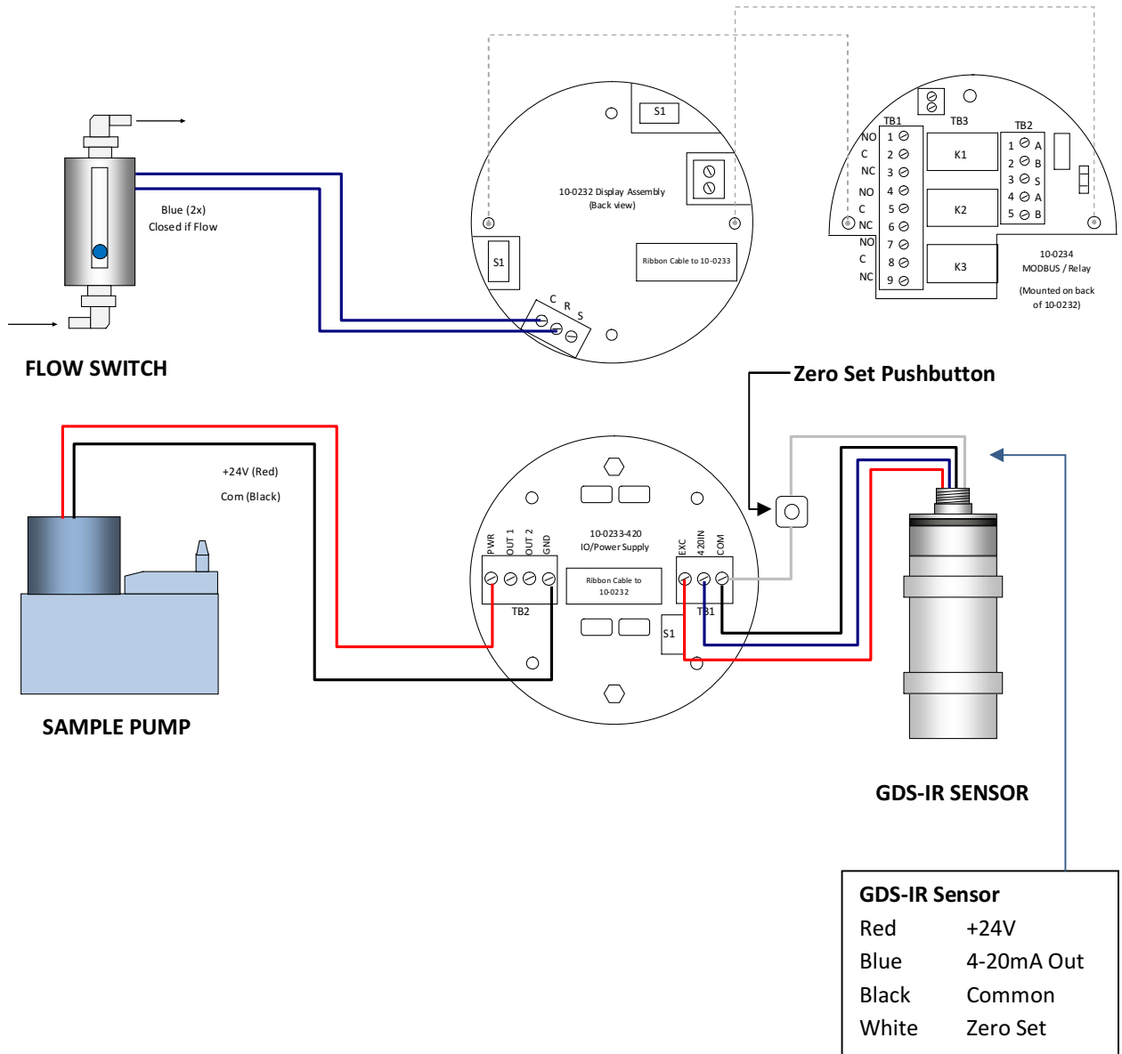
Figure 14-3: GDS-58XP Wiring Diagram (GDS-IR Sensor)
