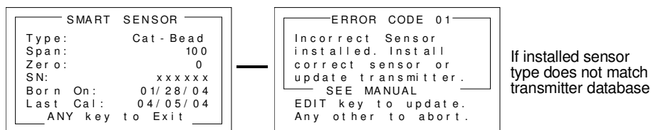
Figure 7-3: Smart Sensor Identification
