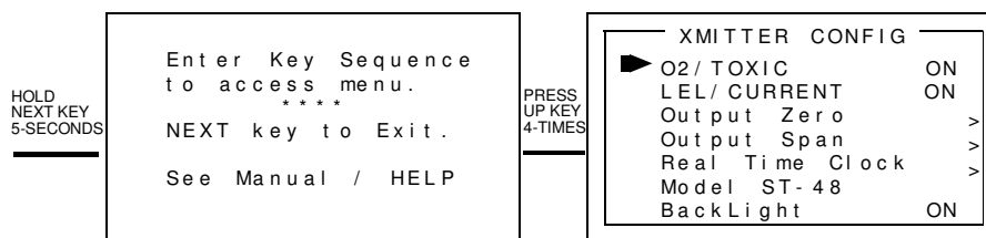
Figure 9-1: XMITTER CONFIG MENU
