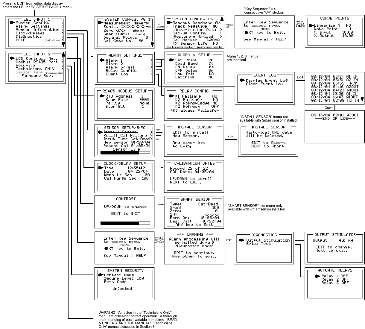
Figure 8-1: MAIN MENU FLOWCHART
