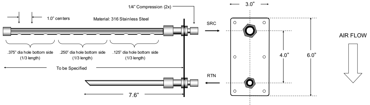
Figure 15-1: Sample Draw Duct Assembly
