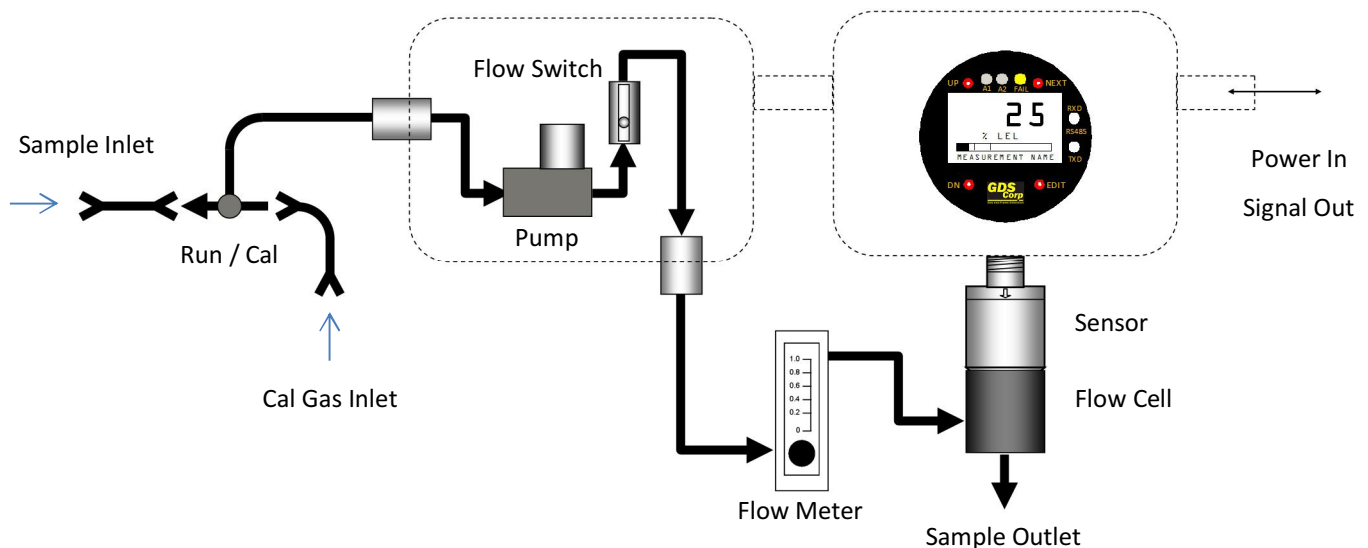
Figure 4-1: GDS-58XP Flow Diagram
