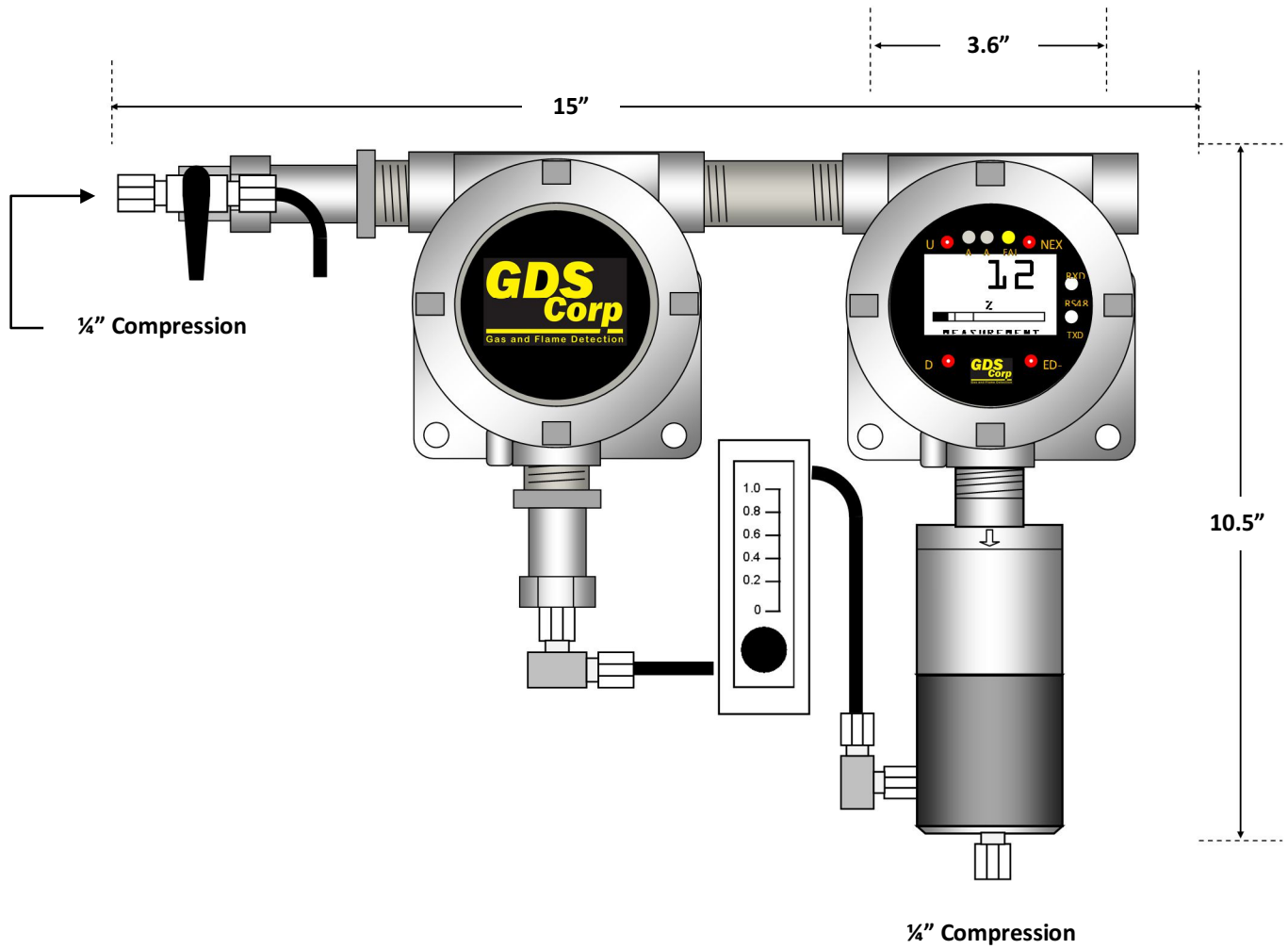
Figure 13-2: GDS-58XP Dimensions (Stainless Steel Enclosure)
