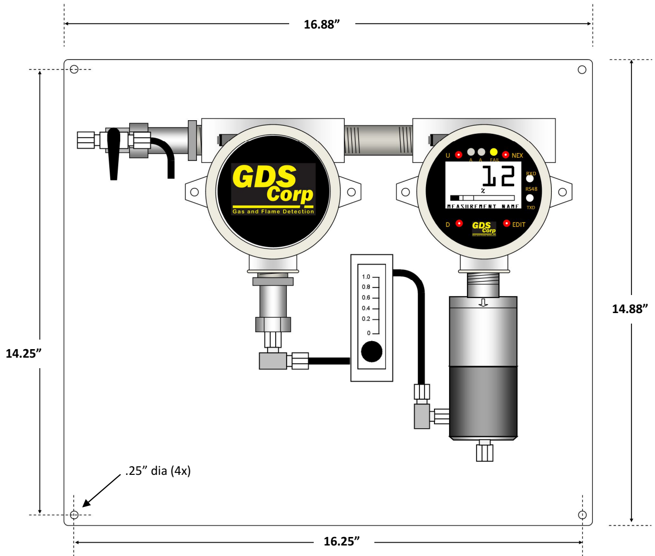
Figure 13-3: GDS-58XP 17" x 15" Mounting Plate Dimensions
