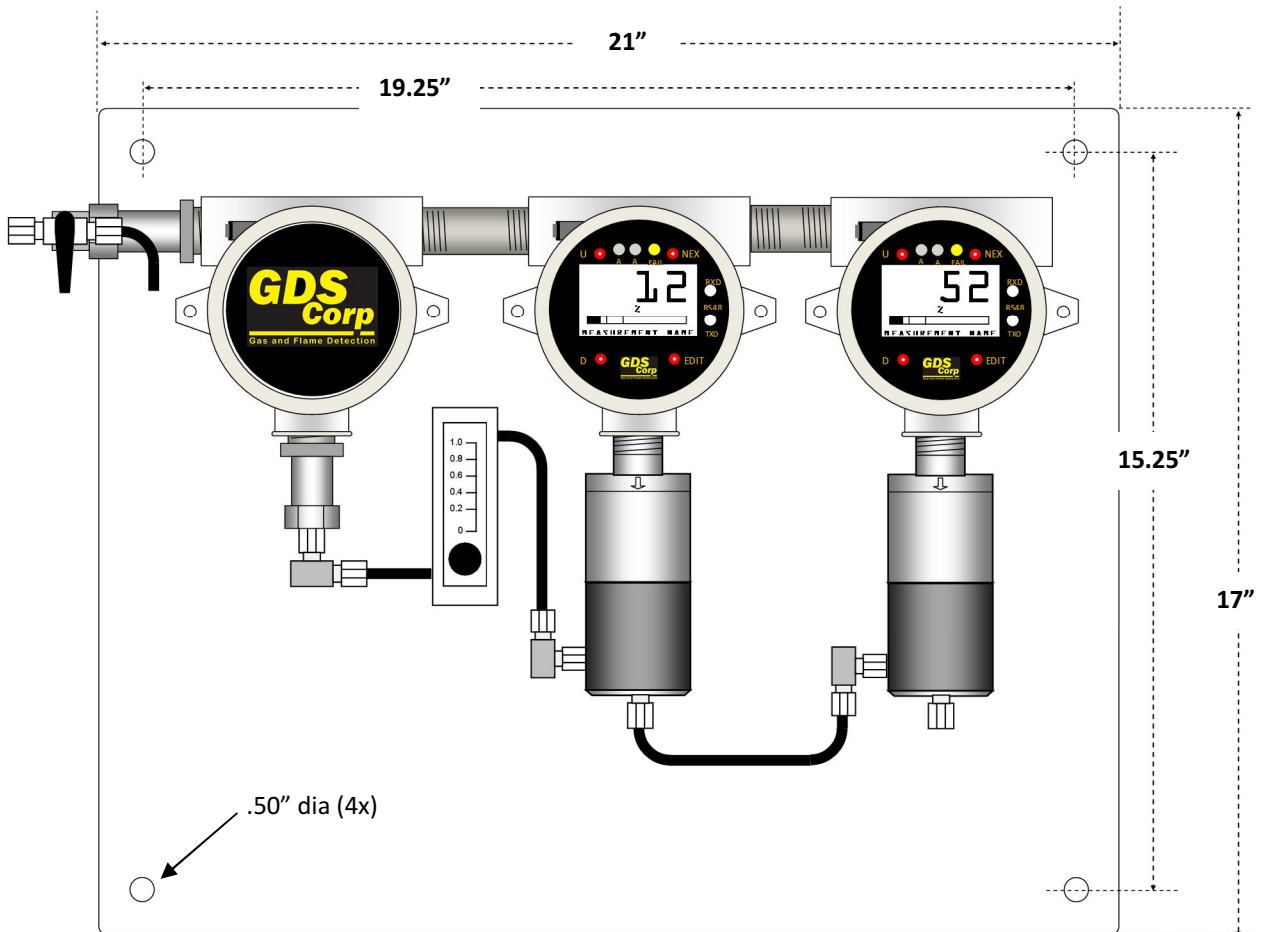
Figure 13-4: GDS-68XP 21" x 17" Mounting Plate Dimensions (AL Enclosures)
