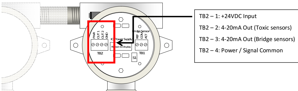
Figure 5-4: GDS-58XP Power & Signal Wiring
