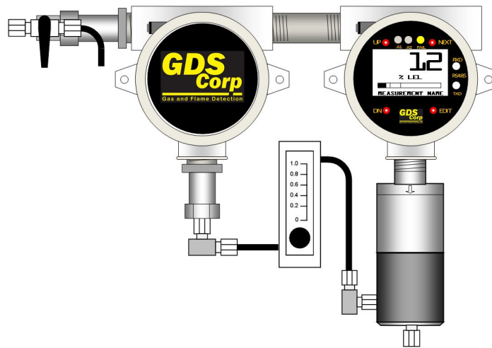
Figure 5-3: GDS-58XP with Toxic Sensor
