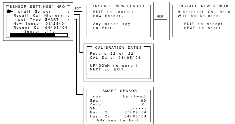
Figure 8-5: SENSOR SETTINGS MENU
