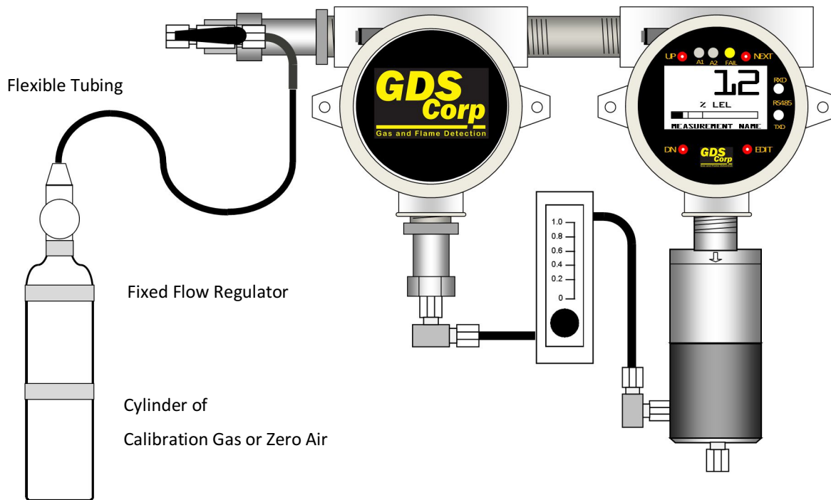
Figure 6-1: GDS-58XP Calibration Setup
