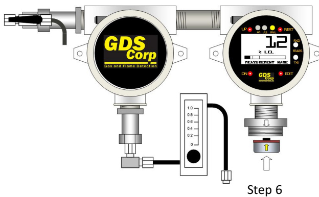
Figure 7-4: Sensor Replacement
