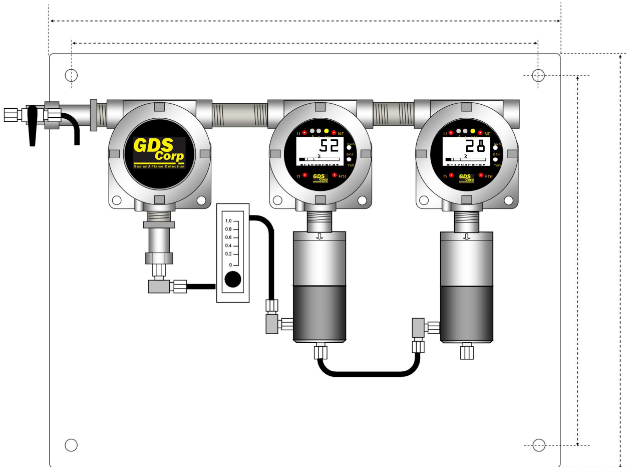
Figure 13-5: GDS-58XP 21" x 17" Mounting Plate Dimensions (SS Enclosures)
