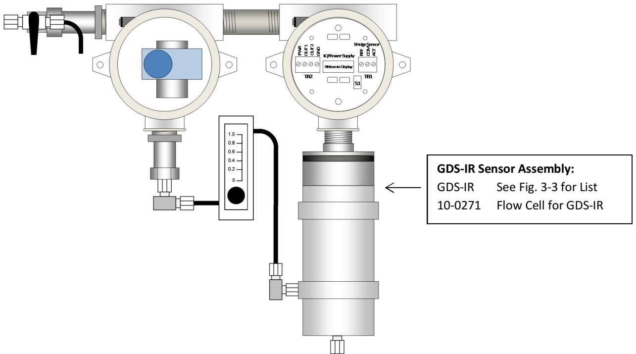
Figure 12-3: GDS-58XP Assembly with GDS-IR (Spare Parts)
