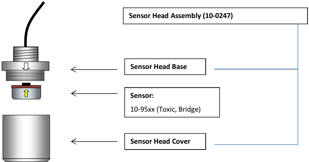
Figure 12-2: GDS-58XP Standard Sensor Head Exploded View
