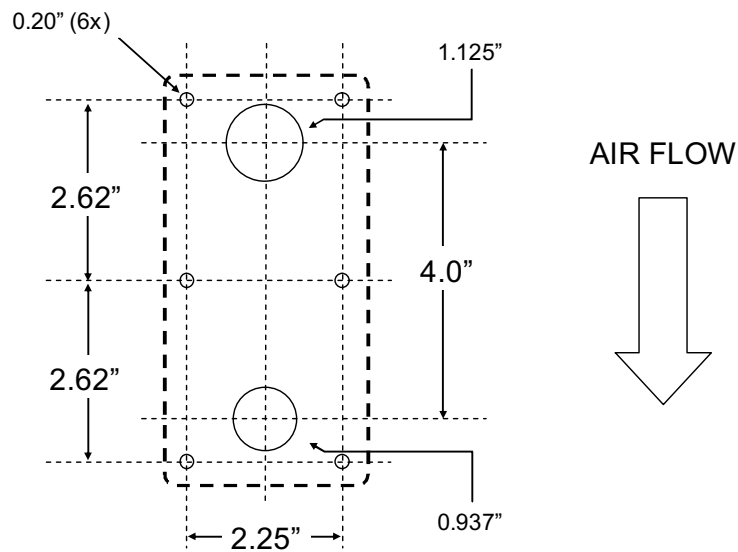
Figure 15-2: Sample Draw Duct Assembly Hole Mounting Pattern
