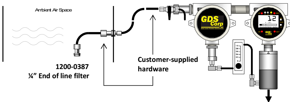
Figure 5-1: GDS-58XP Ambient Air Sampling
