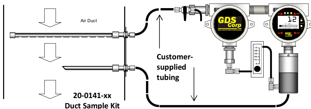
Figure 5-2: GDS-58XP Air Duct Sampling
