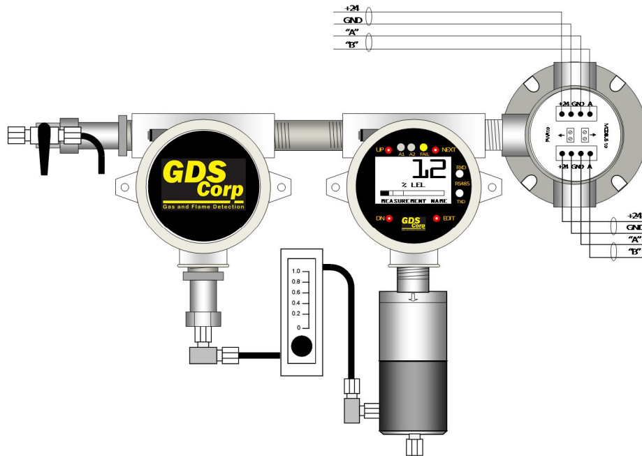
Figure 5-8: GDS-58XP with MODBUS Wiring Junction Box [MBJB]
