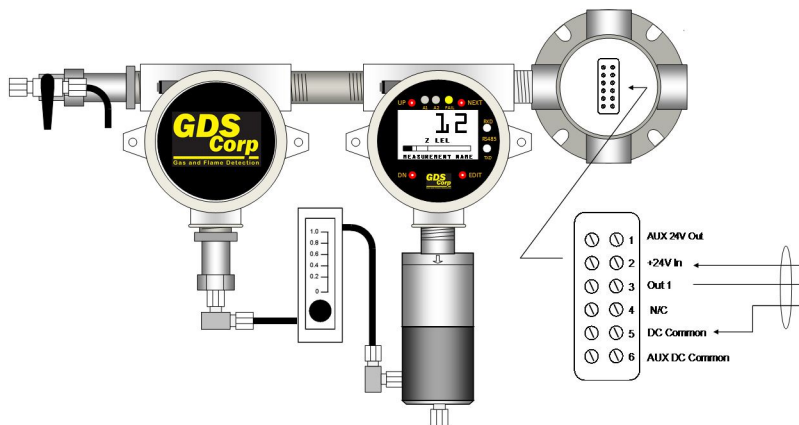
Figure 5-6: GDS-58XP with Analog Wiring Junction Box [RWJB]
