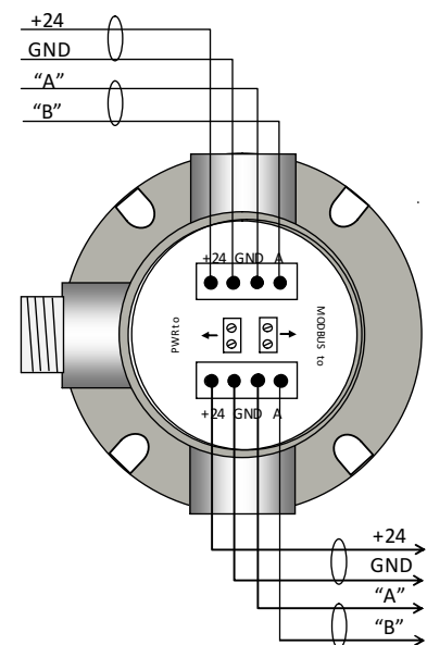
Figure 5-7: MODBUS Wiring Junction Box
