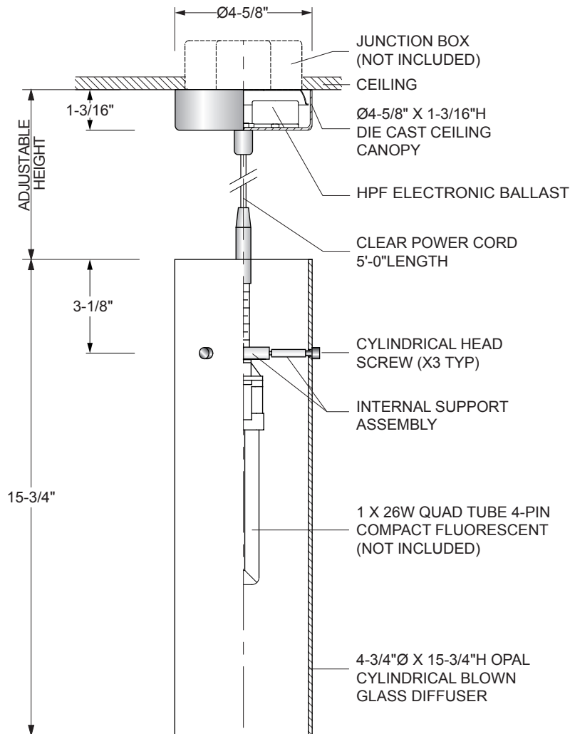
ELEVATION VIEW
