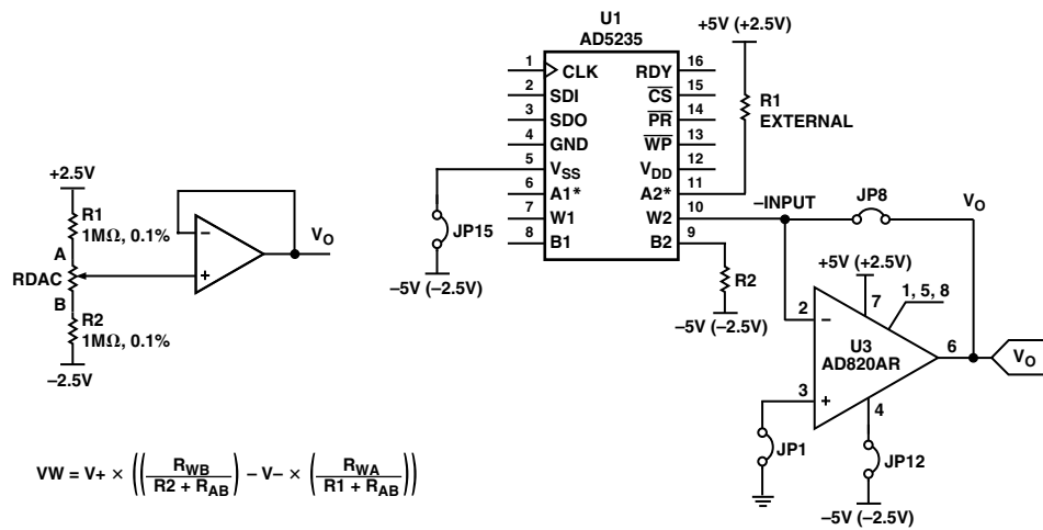
Figure 14. Ultrafine Adjustment
