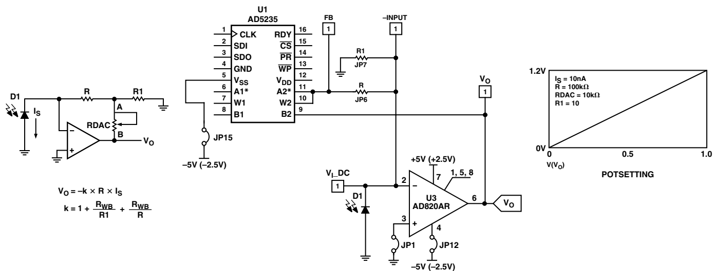
Figure 6. High Sensitivity I-V Coverter
