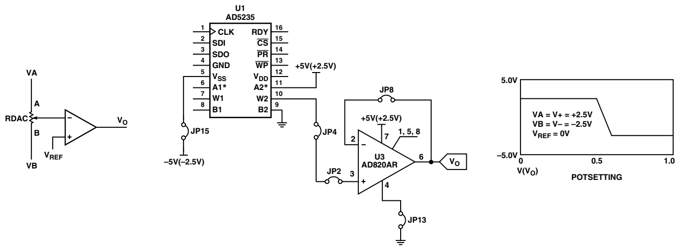
Figure 16. Level Detector
