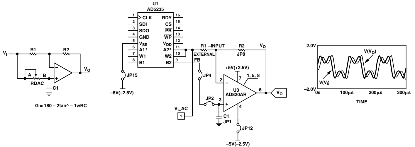
Figure 15. Phase Shifter
