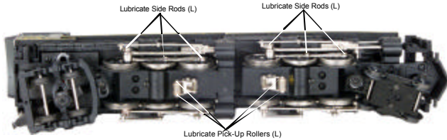
Figure 2. Lubrication Points on the Engine
