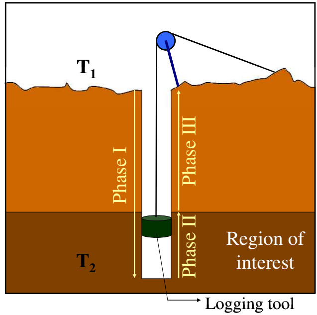
Figure 1. Schematic of wireline logging application
