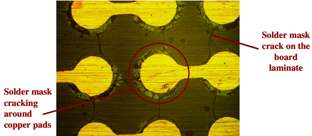
Figure 29. Lateral section of Sn based finish Sn3.5Ag solder Board2 – Package G (256 I/O BGA) (courtesy: CALCE)
