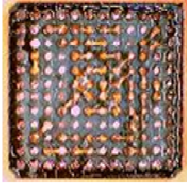
Figure 27. Optical picture of the pried 144 I/O BGA package in Sn based finished Sn3.5Ag soldered board (courtesy: CALCE)
