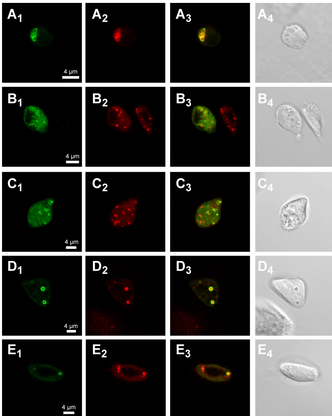
FIG. 3. Subcellular localization of representative lipid droplet-associated proteins in Drosophila S2 cells. A, lipid droplet association of fluorescently tagged PAT domain proteins (A 1 , LSD-1-EGFP; A 2 , LSD-2-red fluorescent protein; A 3 , merged channels A 1 + A 2 ; A 4 , differential interference contrast). B and C, localization of CG1112-EGFP (B 1 ) and CG10691-EGFP (C 1 ) at a subset of lipid droplets (B 2 and C 2 ) and in the cytoplasm (merged channels, B 3 and C 3 ; differential interference contrast images, B 4 and C 4 ). D and E, specific CG2254-EGFP localization (D 1 and E 1 ) around lipid droplets (D 2 and E 2 ; merged channels, D 3 and E 3 ; differential interference contrast images, D 4 and E 4 ). Note that CG2254-EGFP decorates a subset of lipid droplets in E. Lipid droplets are visualized by Nile Red stain in B–E.
